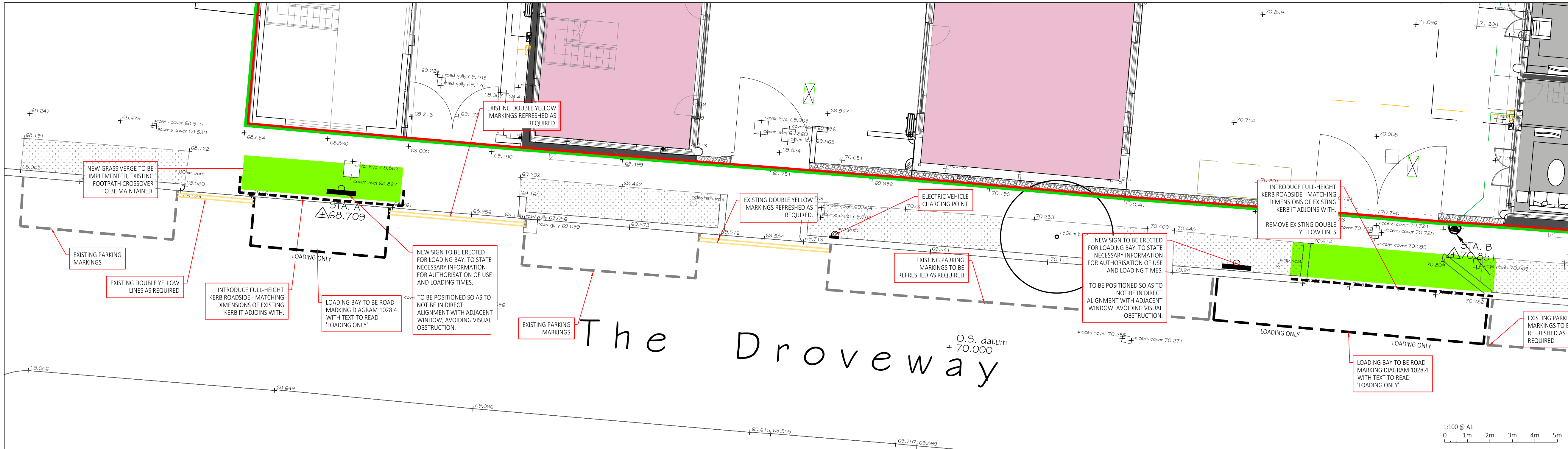
PROPOSED SIGNS AND ROAD MARKINGS (1:100)
